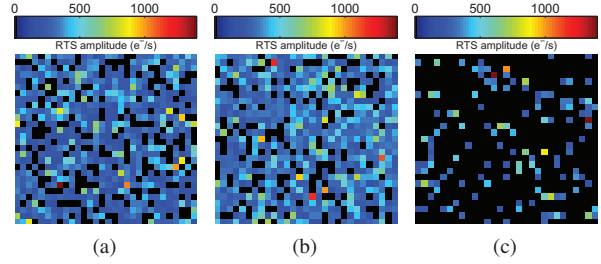
Fig. 12. Mappings of detected RTS pixels amplitudes after 30 krad for the three studied pixel layouts: (a) standard, (b) standard with ELT in-pixel MOSFETs, (c) recessed field oxide and ELT in-pixel MOSFETs.
